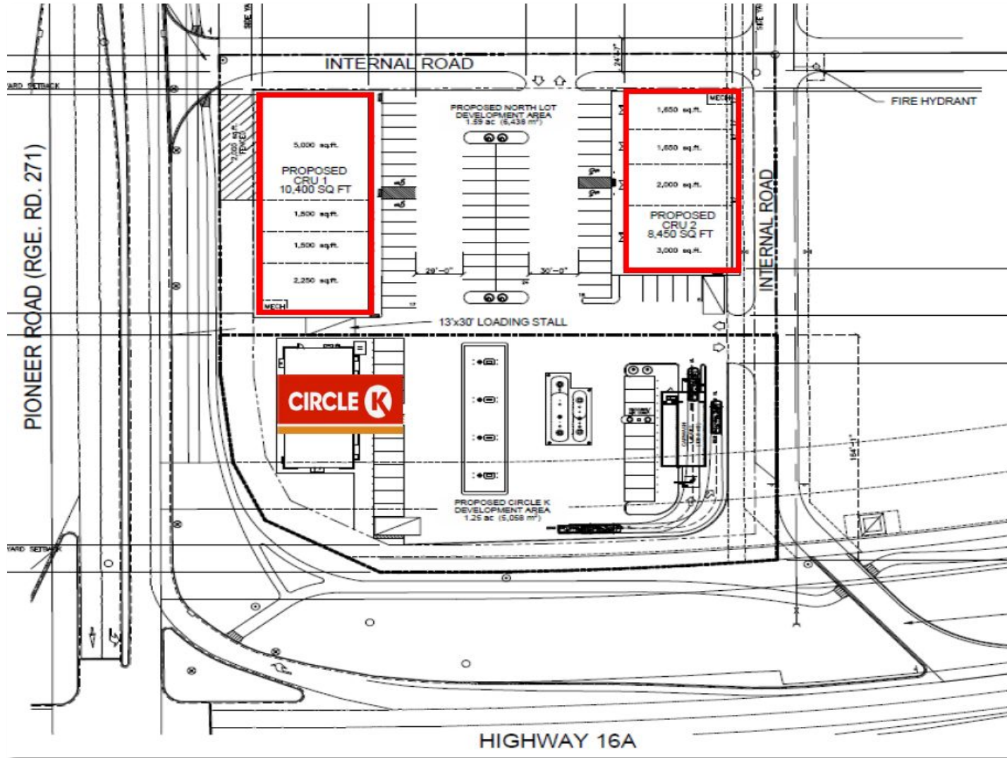
Decker Properties Management Ltd. commercial development sites 4a & 4b
